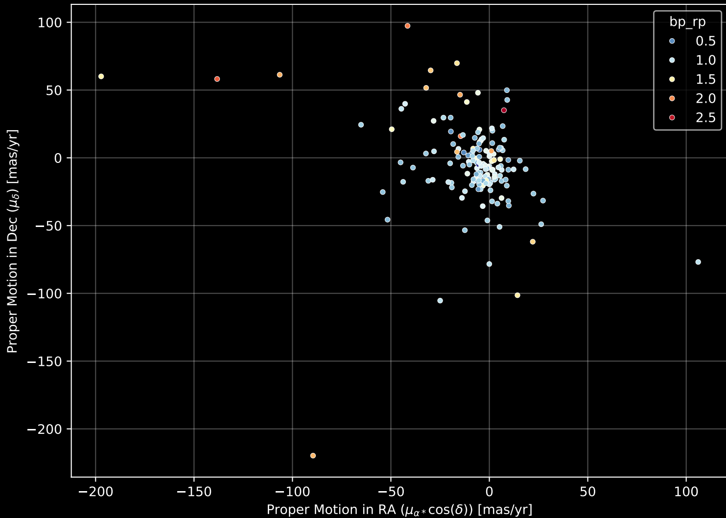
APOGEE DR17 Field: [063+41_MGA] Proper Motion Diagram (n= 162)
