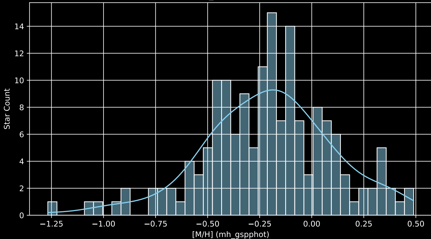
APOGEE DR17 Field: [063+41_MGA [M/H] (mh_gspphot) (n= 161)
