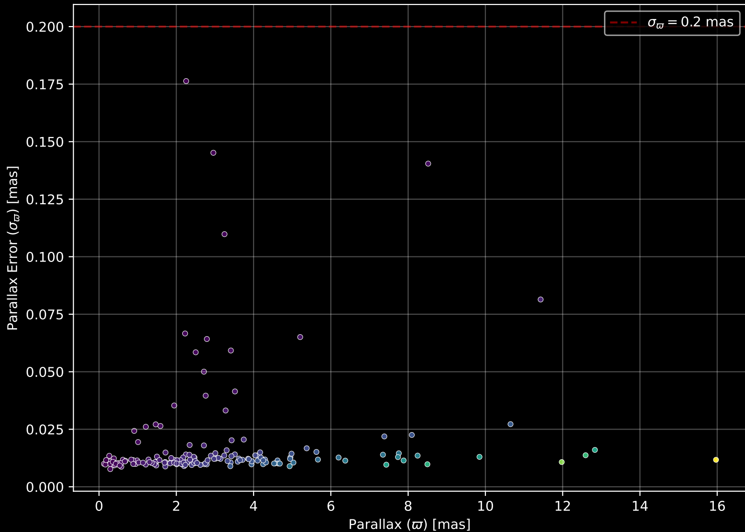
APOGEE DR17 Field: [063+41_MGA] Parallax Quality (n= 162)
