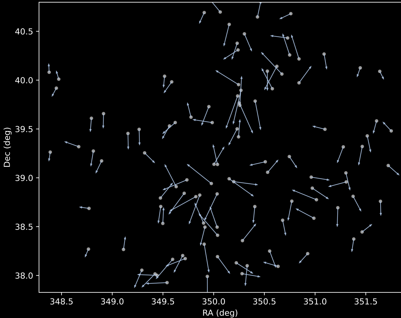
APOGEE DR17 Cluster 1 Proper Motion Vectors (n=108)
