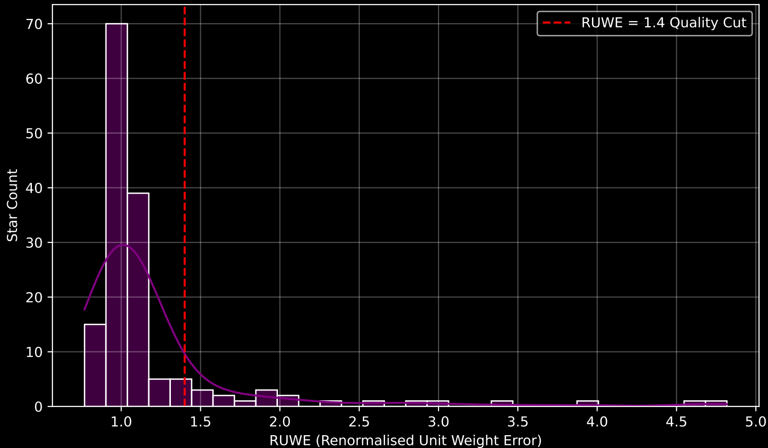
GAPOGEE DR17 Field [063+41_MGA] RUWE Distribution (n= 153)
