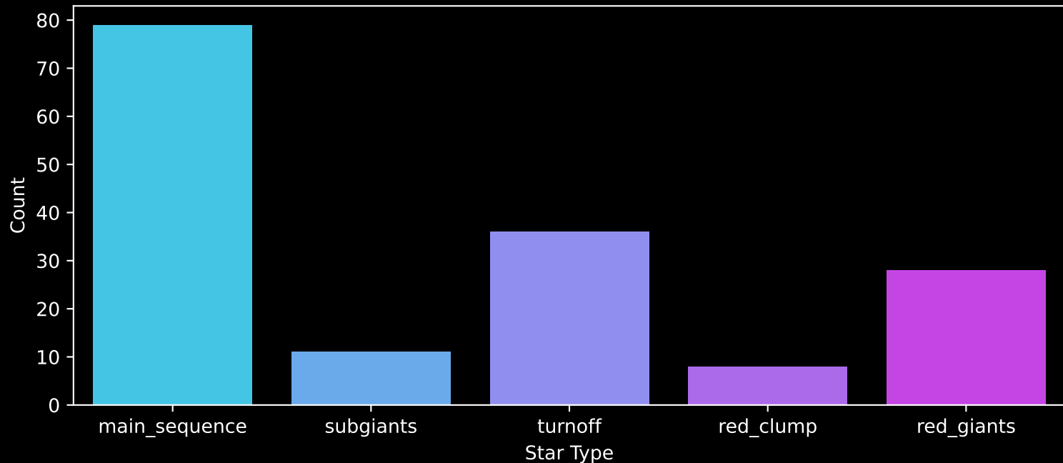
APOGEE DR17 Field: [063+41_MGA] Count plot of Star Type
